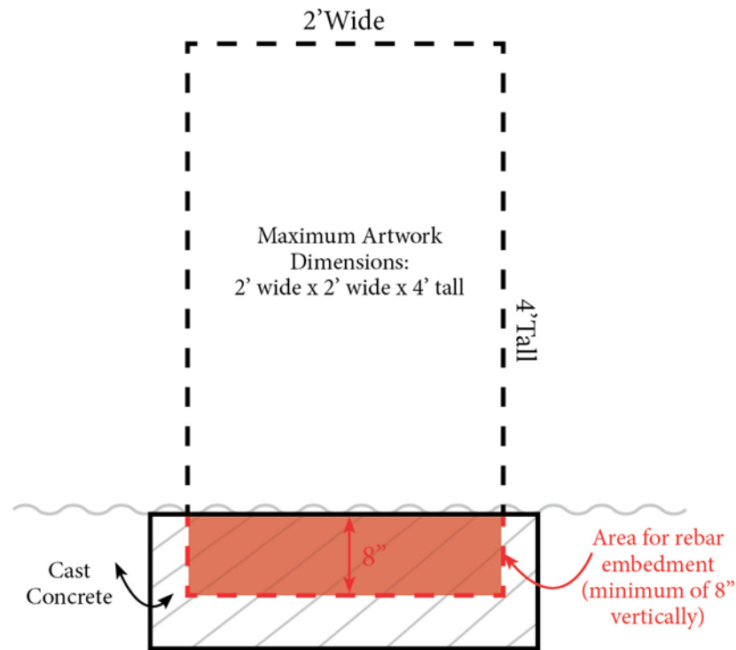
*DIAGRAM of rebar to be anchored in 12" of concrete (Not to Scale).
